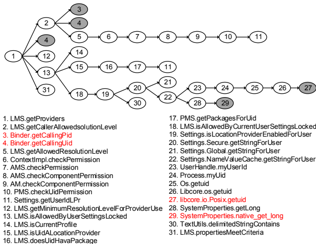
Fig. 9. Sub-call graph rooted at getProviders() . (LMS, AM, AMS, and PMS represent LocationManagerService , ActivityManager , ActivityManagerService , and PackageManagerService , respectively. The grey nodes denote native methods.)
