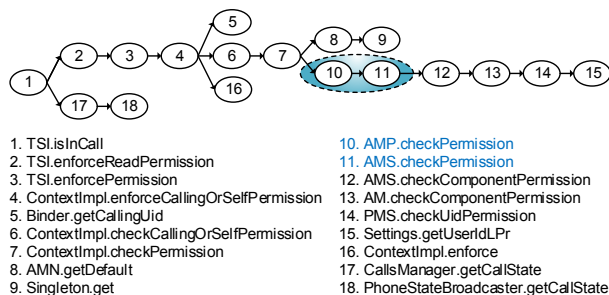
Fig. 11. Sub-call graph rooted at isInCall() . ( TSL , AMN , AMP , AMS , and PMS represent TelecomServiceImpl , ActivityManagerNative , ActivityManagerProxy , ActivityManagerService , and PackageManagerService , respectively. The blue area denotes an IPC service call made through Binder .)
